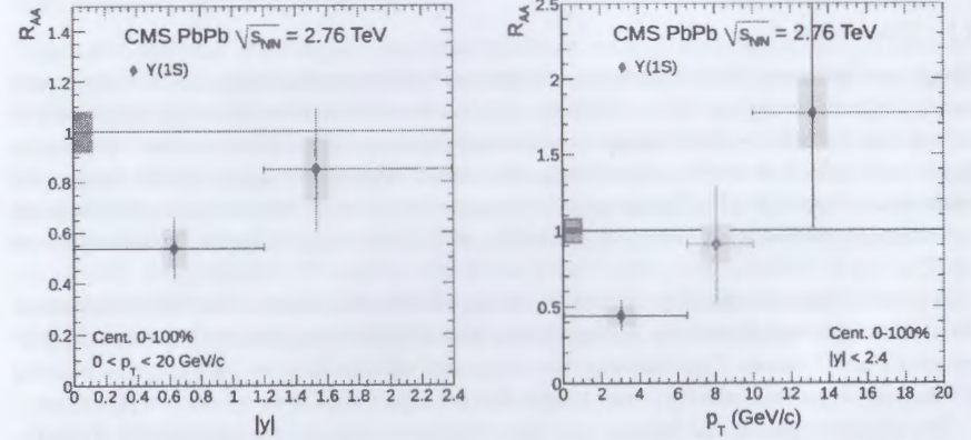
Figure 10: Nuclear modification factor R_{AA} of \Upsilon(1S) as a function of rapidity (left) and p_T (right). A global uncertainty of 8.3%, from T_{AA} and the integrated luminosity of the pp data sample, is shown as a grey box at R_{AA} = 1 . Points are plotted at their measured average p_T . Statistical (systematic) uncertainties are shown as bars (boxes). Horizontal bars indicate the bin width.
