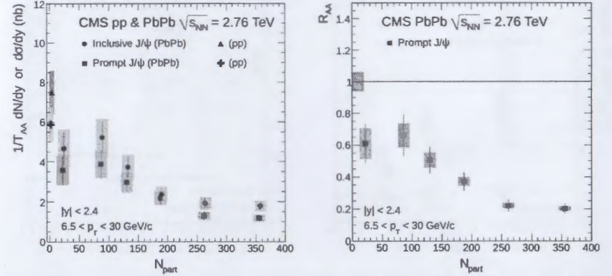
Figure 6: Left: yield of inclusive J/\psi (blue circles) and prompt J/\psi (red squares) divided by T_{AA} as a function of N_{part} . The results are compared to the cross sections of inclusive J/\psi (black triangle) and prompt J/\psi (black cross) measured in pp. The inclusive J/\psi points are shifted by \Delta N_{part} = 2 for better visibility. Right: nuclear modification factor R_{AA} of prompt J/\psi as a function of N_{part} . A global uncertainty of 6%, from the integrated luminosity of the pp data sample, is shown as a grey box at R_{AA} = 1 . Statistical (systematic) uncertainties are shown as bars (boxes).
