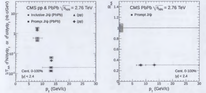
Figure 7: Left: yield of inclusive J/\psi (blue circles) and prompt J/\psi (red squares) divided by T_{AA} as a function of p_T . The results are compared to the cross sections of inclusive J/\psi (black triangles) and prompt J/\psi (black crosses) measured in pp. The global scale uncertainties on the PbPb data due to T_{AA} (5.7%) and the pp integrated luminosity (6.0%) are not shown. Right: nuclear modification factor R_{AA} of prompt J/\psi as a function of p_T . A global uncertainty of 8.3%, from T_{AA} and the integrated luminosity of the pp data sample, is shown as a grey box at R_{AA} = 1 . Points are plotted at their measured average p_T . Statistical (systematic) uncertainties are shown as bars (boxes). Horizontal bars indicate the bin width.
