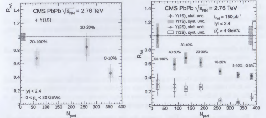
Figure 11: Nuclear modification factor R_{AA} of \Upsilon(1S) (left) and both 1S+2S (right) states as a function of N_{part} . A global uncertainty of 6%, from the integrated luminosity of the pp data sample, is shown as a grey box at R_{AA} = 1 . Statistical (systematic) uncertainties are shown as bars (boxes).
